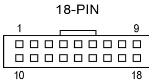
18-pin I/O connector (looking at the acceptor)
